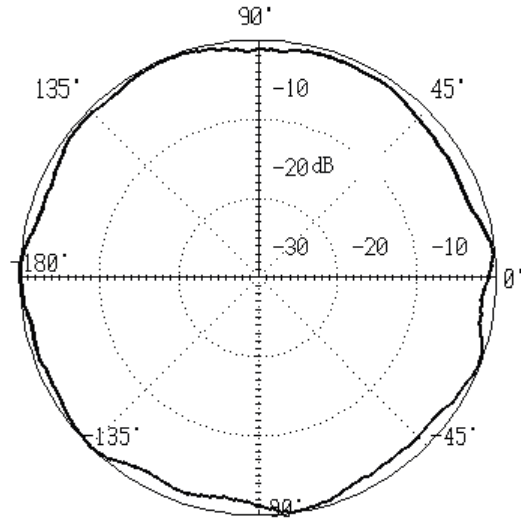
H Plane
