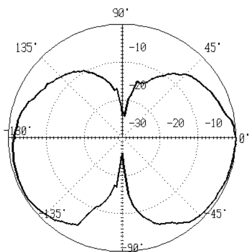
E Plane
